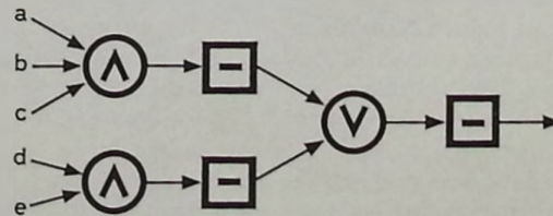
Abb. 2c \overline{(\overline{a \wedge b \wedge c}) \vee (\overline{d \wedge e})}
